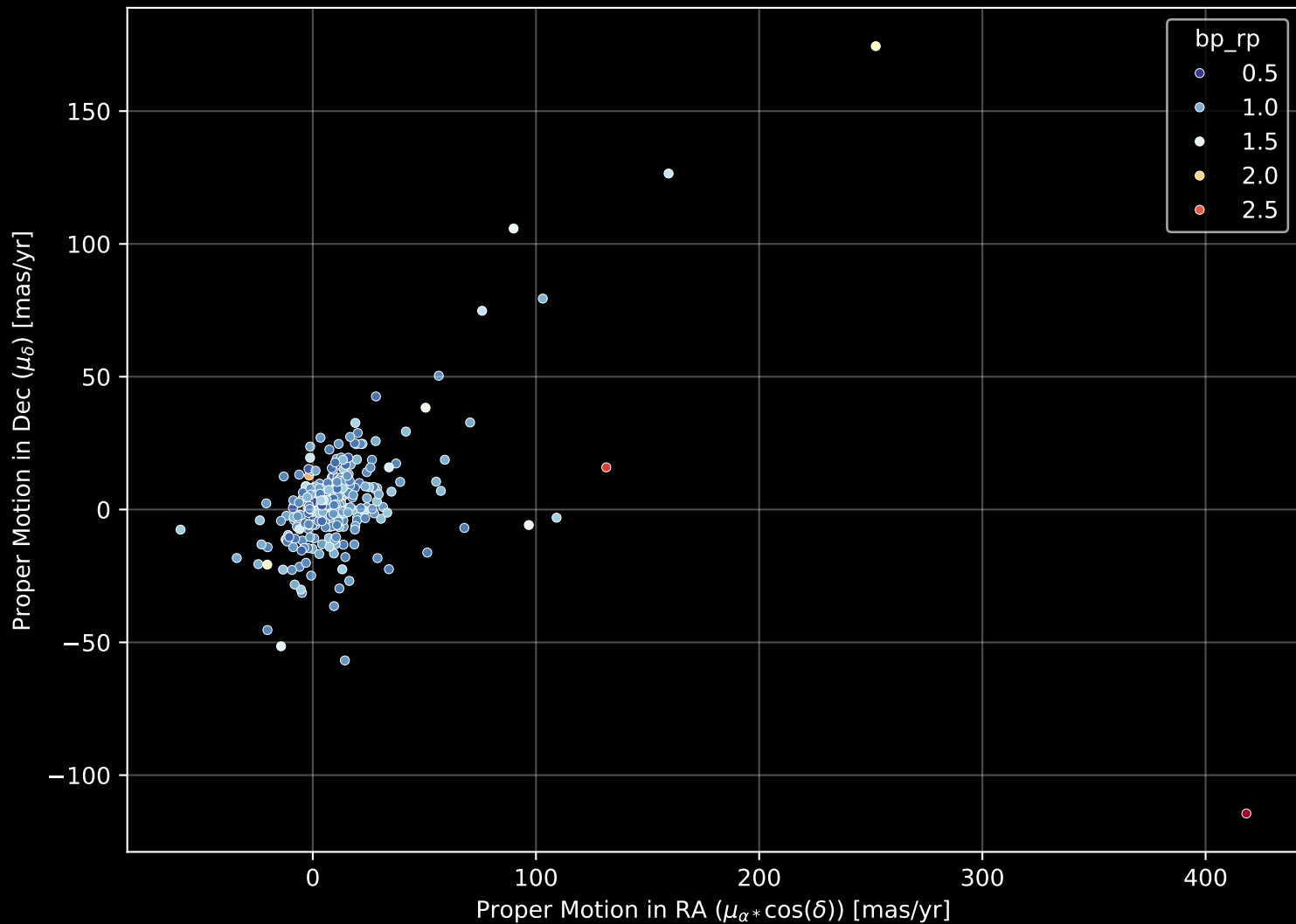
GALAH DR4 Field: [7005] Proper Motion Diagram (n= 299)
