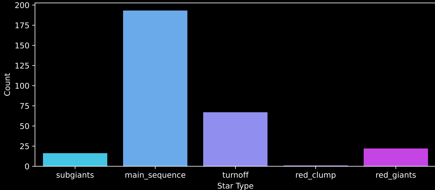
GALAH DR4 Field: [7005] Count plot of Star Type
