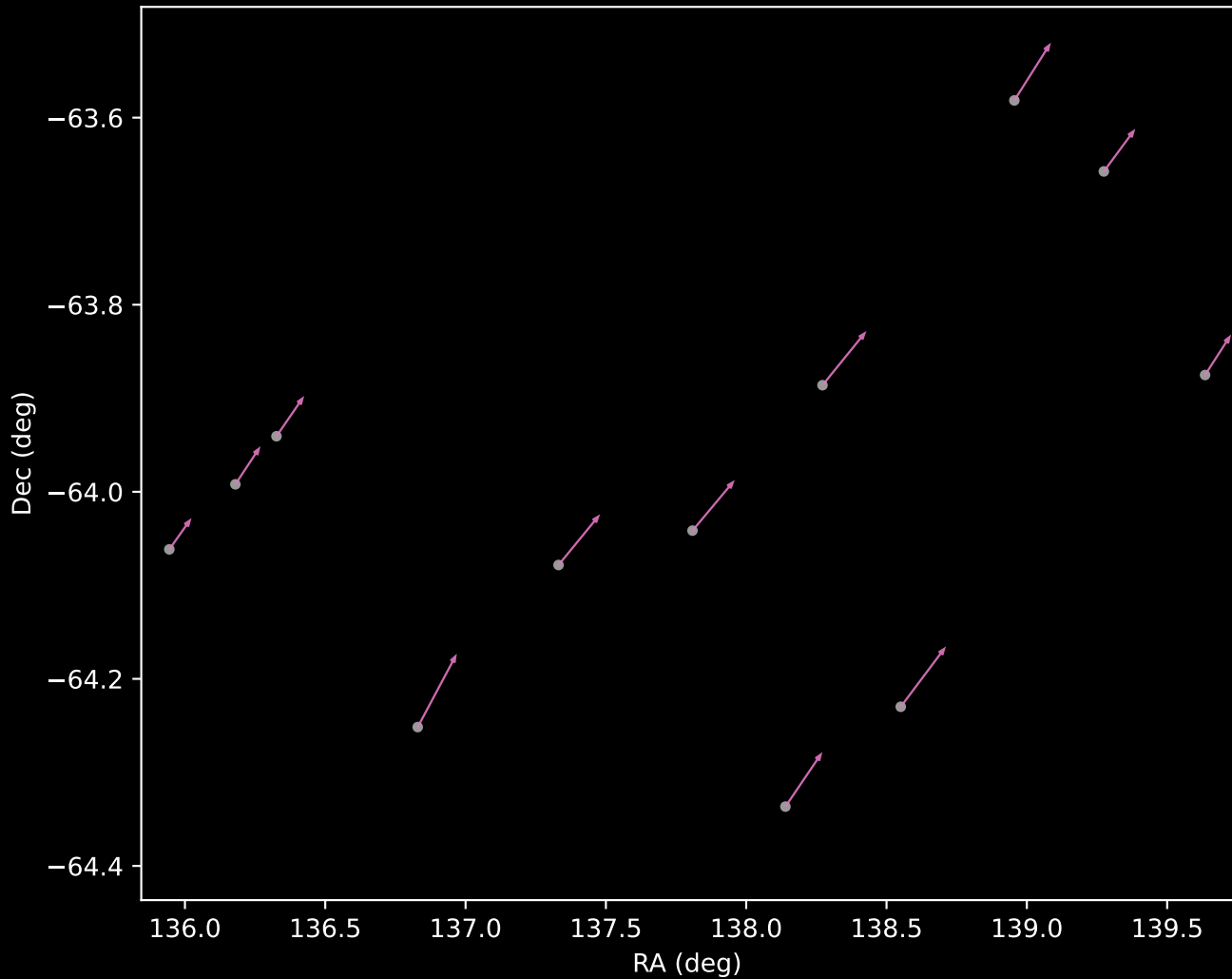
GALAH DR4 Cluster 12 Proper Motion Vectors (n=12)
