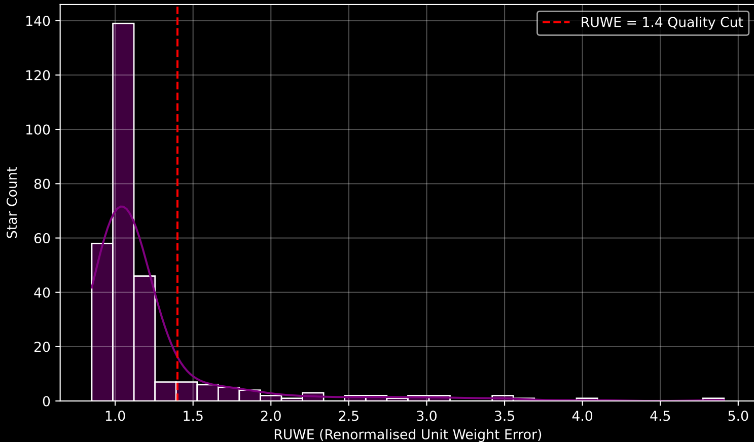
GALAH DR4 Field [7005] RUWE Distribution (n= 292)
