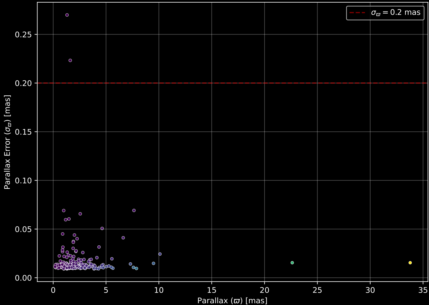
GALAH DR4 Field: [7005] Parallax Quality (n= 299)
