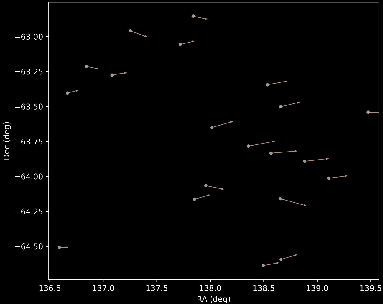
GALAH DR4 Cluster 11 Proper Motion Vectors (n=20)
