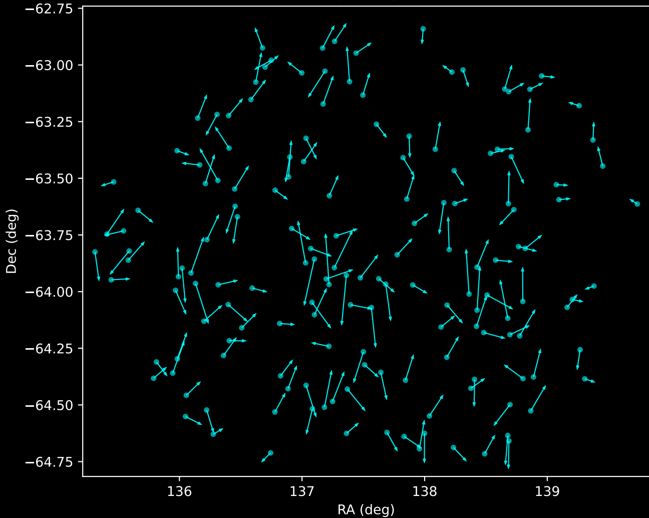
GALAH DR4 Noise Stream Proper Motion Vectors (n=158)
