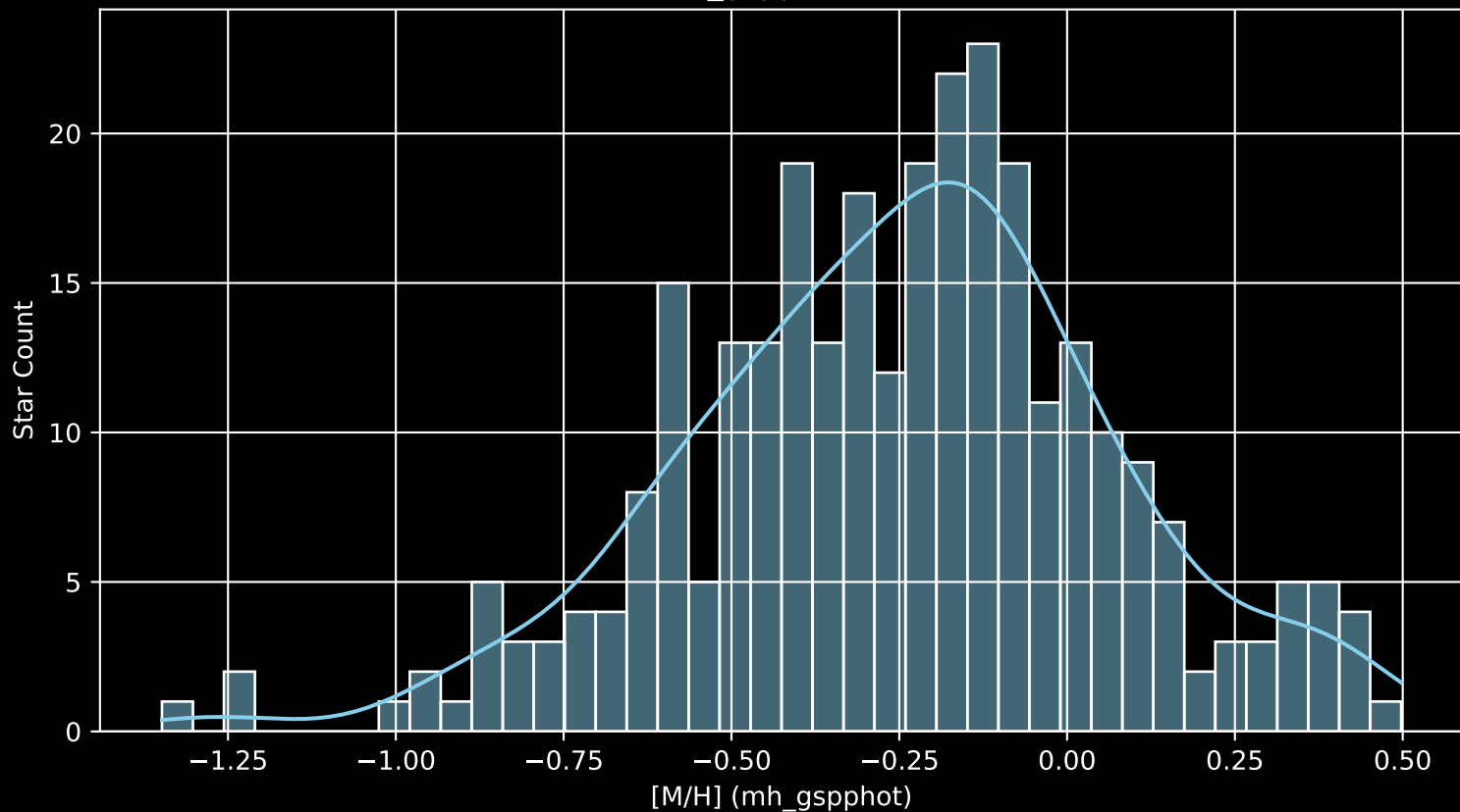
GALAH DR4 Field: [7005] [M/H] (mh_gspphot) (n= 298)
